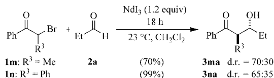
Scheme 2. Diastereoselectivity in NdI 3 -mediated Reformatsky-type reactions.
