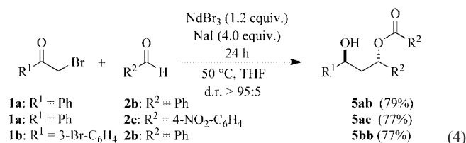
Scheme 3. Plausible mechanism through neodymium(III) enolates.
