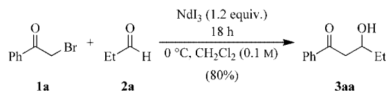
Scheme 1. Formation of 3aa from 1a and 2a in the presence of \text{NdI}_3 .
