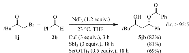
Scheme 4. NdI 3 -mediated aldol–Tishchenko reactions in the presence of additives.
